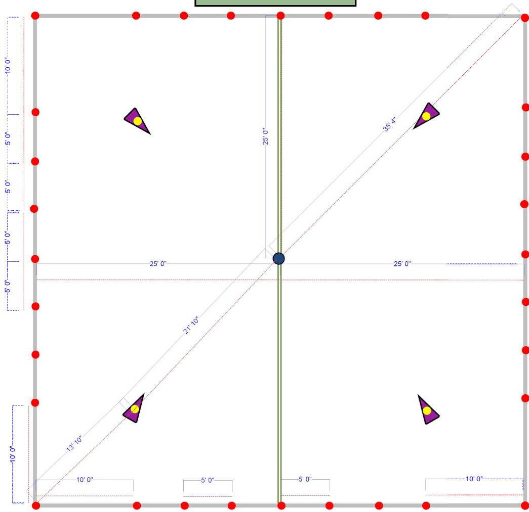
50' x 50' Pole Tent - Pole Placements
